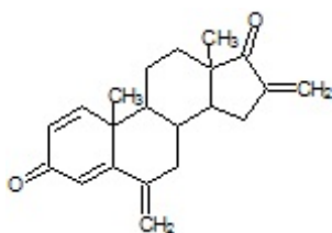
7. 6,16-Dimethylene-1,4-androstadiene-3,17-dione
