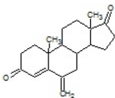
4. 6-Methylene-4-androstene-3-17-dione
